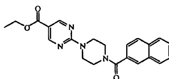
intermediate 12
